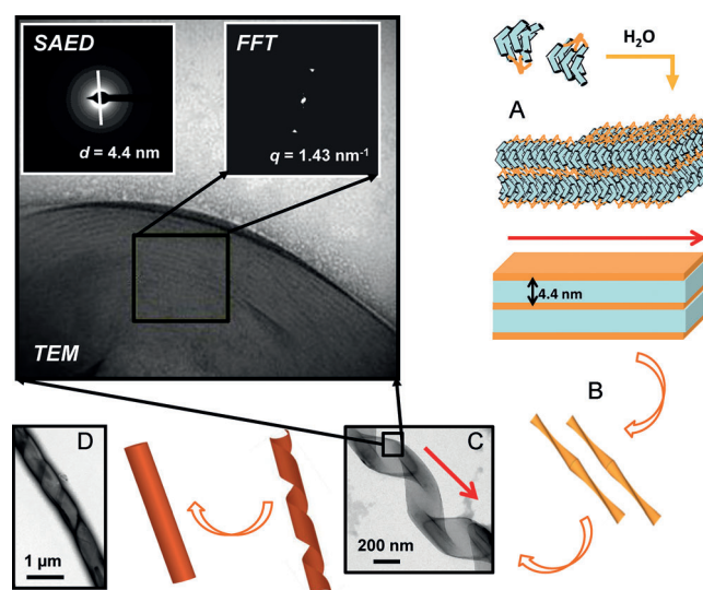
Figure 3. TEM image of PPI1-B1-4-8 showing a lamellar arrangement (insets: selected-area electron diffraction (SAED) and fast Fourier transform (FFT) images) in the helical ribbons and tubes. Proposed mechanism for the hierarchical self-assembly of the ionic dendrimers in the presence of water (A–D).
